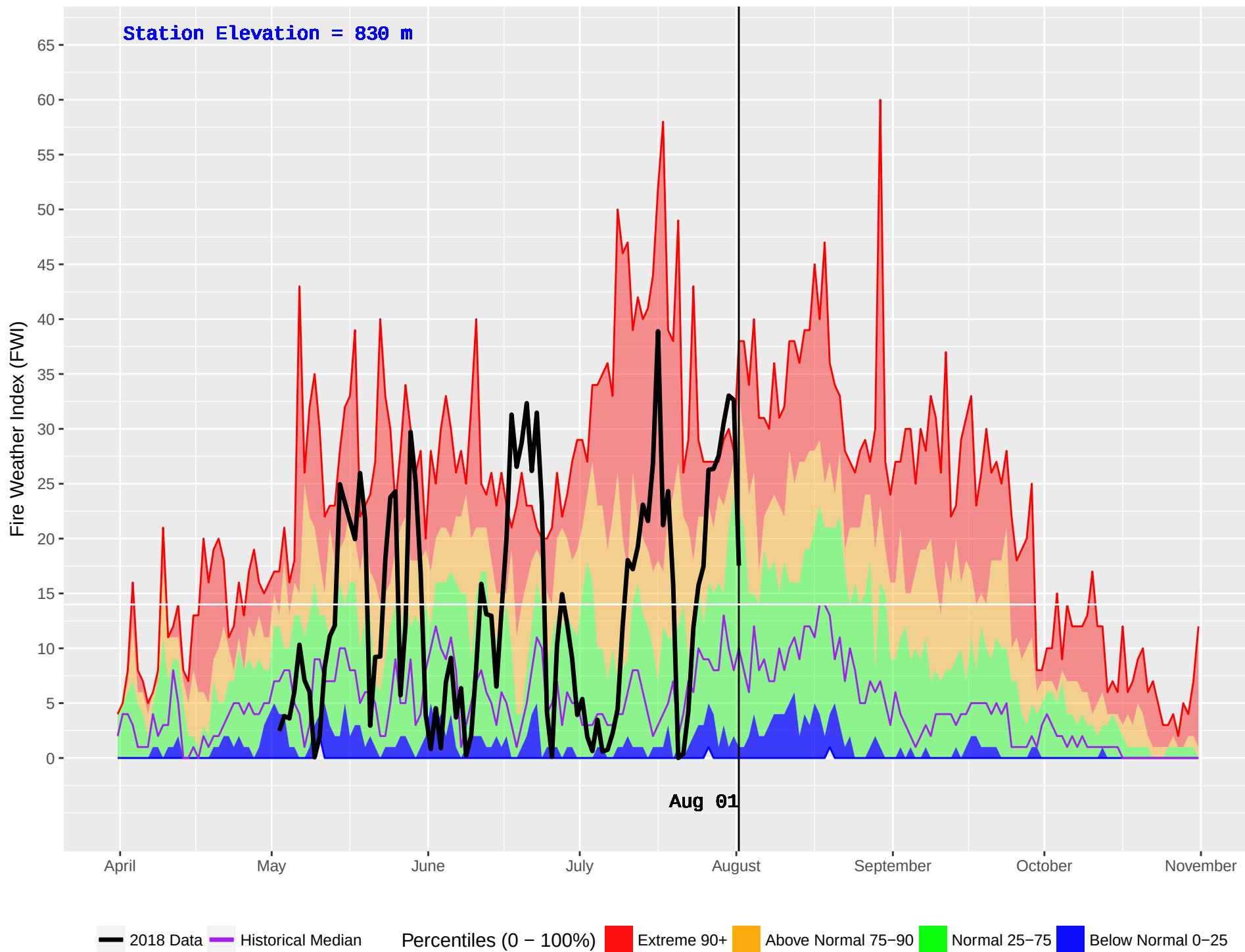
BURNS LAKE 850M (181) : Historical (1993–2016) and Current (2018) Daily Fire Weather Index (FWI)
