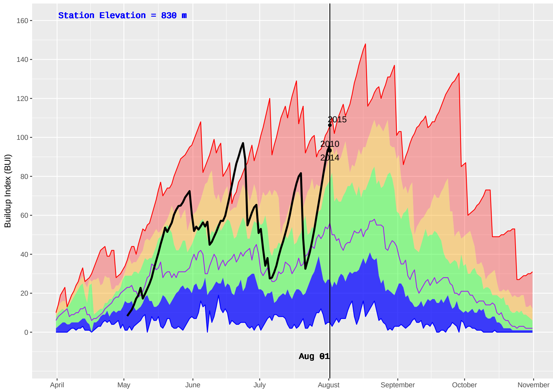
BURNS LAKE 850M (181) : Historical (1993–2016) and Current (2018) Daily Buildup Index (BUI)
