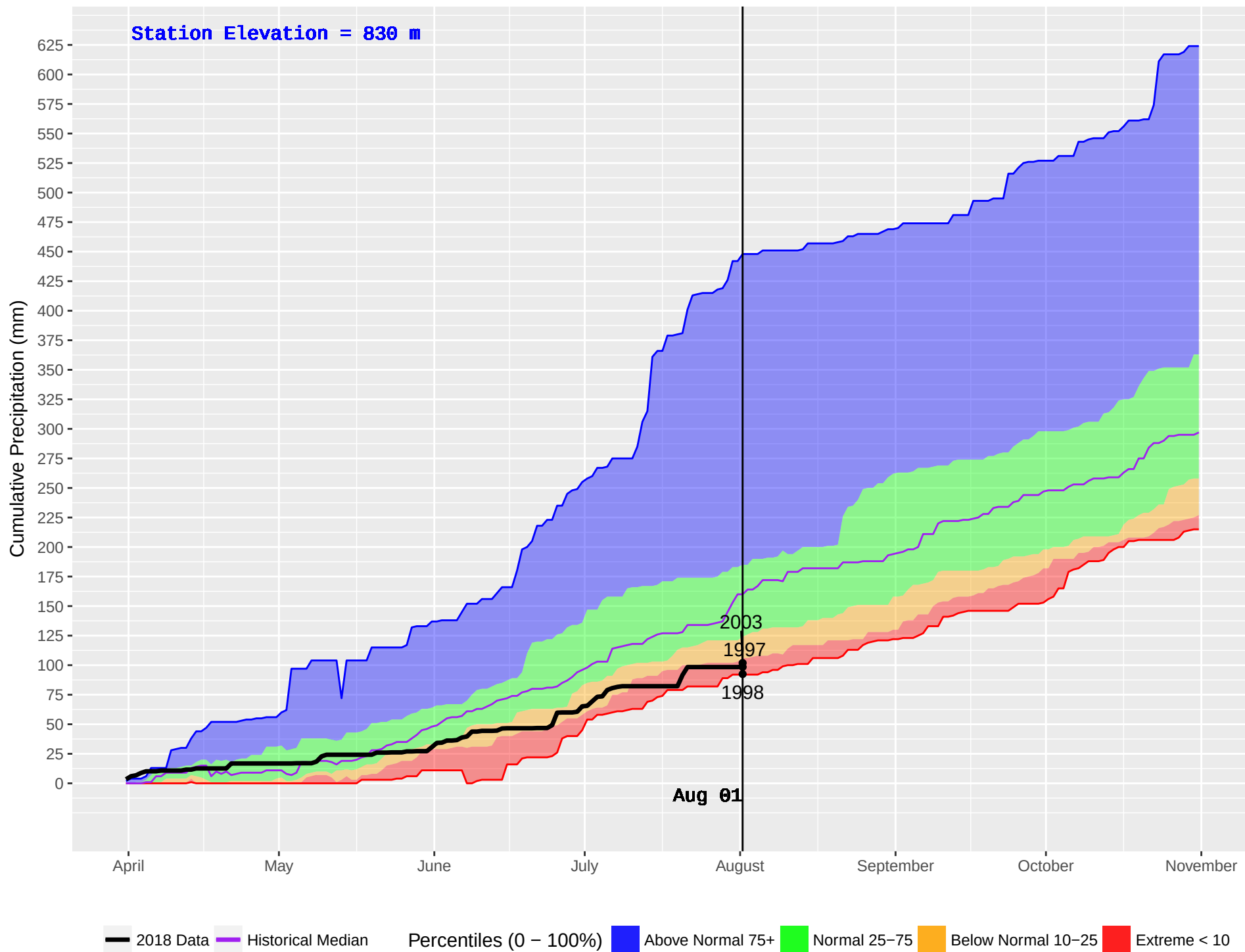
BURNS LAKE 850M (181) : Historical (1993–2016) and Current (2018) Daily Cumulative Precipitation
